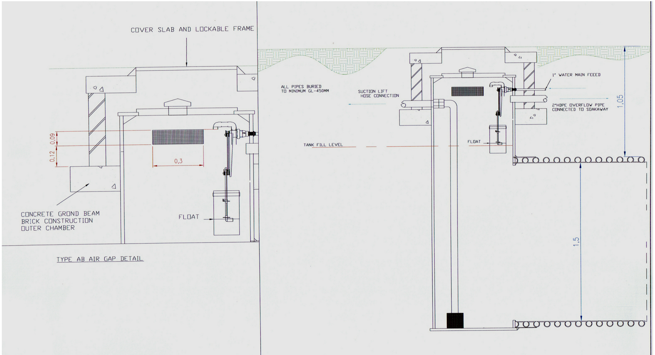
Tank Feed and overflow detail
